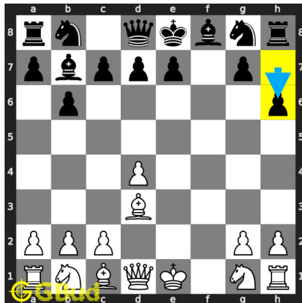
Figure 4: h6
