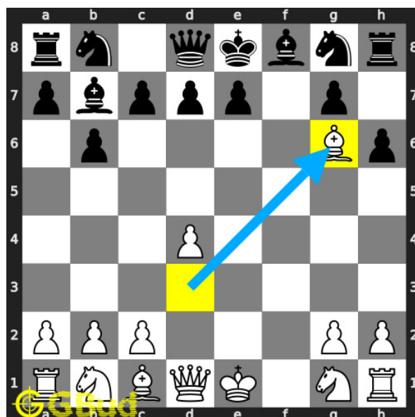
Figure 5: Bg6#
